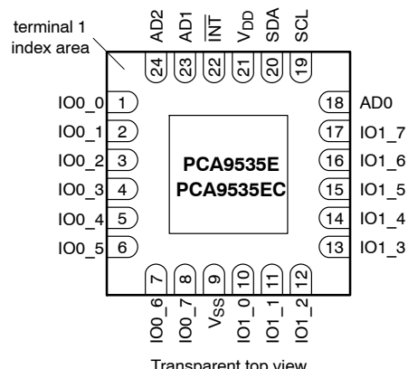
Figure 4. WQFN24
