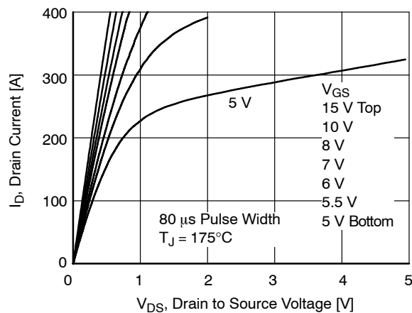
Figure 10. Saturation Characteristics
