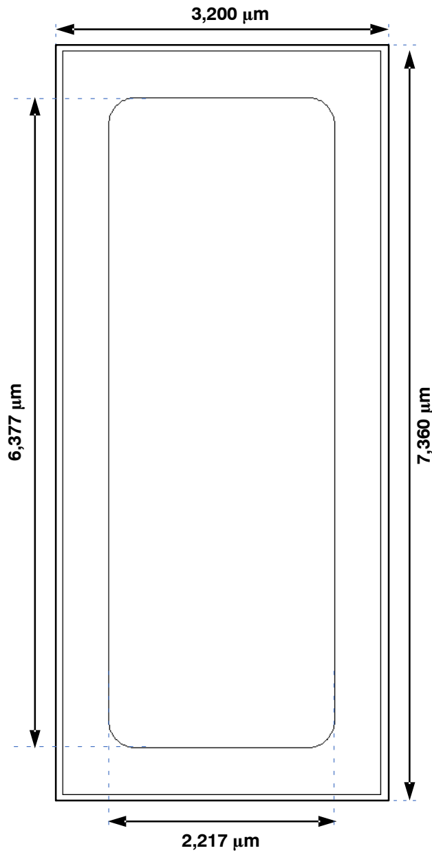
Figure 1. Die Layout
