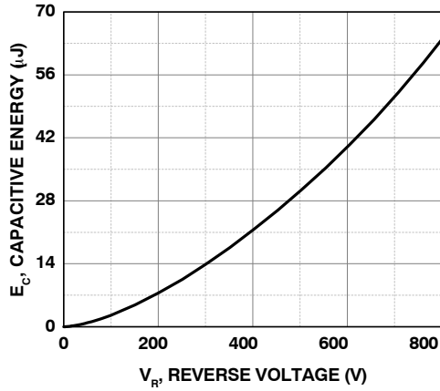
Figure 8. Capacitive Stored Energy
