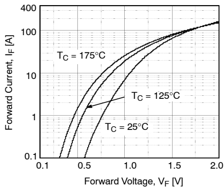
Figure 5. Typical Forward Voltage Drop vs. Forward Current
