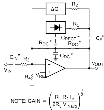
Figure 7. Basic Compressor
