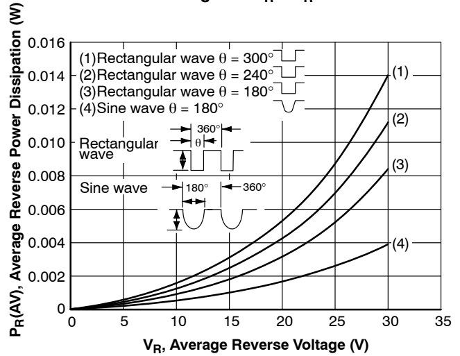
Figure 5. P_R(AV) - V_R
