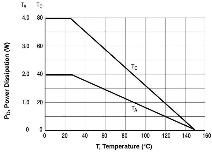
Figure 2. Power Derating
