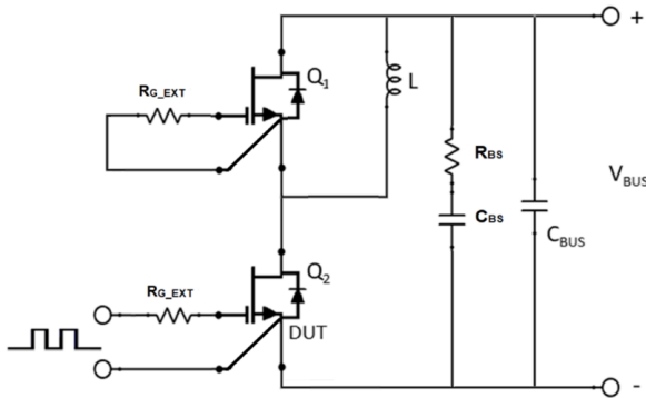
Figure 23. Schematic of the Half-bridge Mode Switching Test Circuit. Note, a Bus RC Snubber ( R_{BS} = 2.5\text{ }^\Omega , C_{BS} = 100\text{ nF} ) is Used to Reduce the Power Loop High Frequency Oscillations
