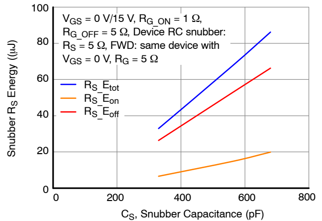
Figure 24. RC Snubber Energy Losses vs. Snubber Capacitance C_S at V_{DS} = 400 V, I_D = 70 A and T_J = 25 °C
