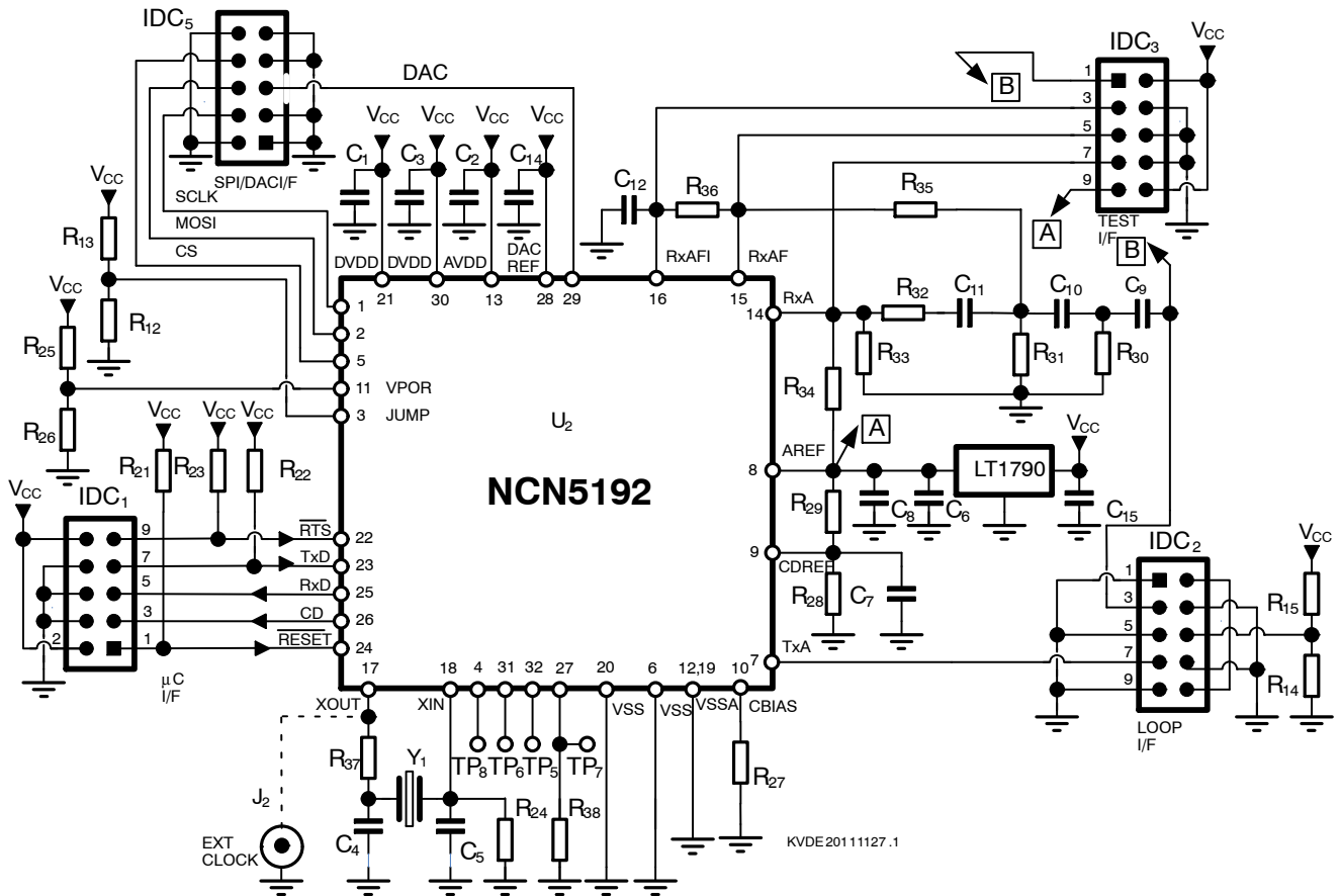
Figure 2. NCN5192NGEVB Schematic
