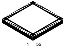
QFN-52 CASE 485M MN SUFFIX
