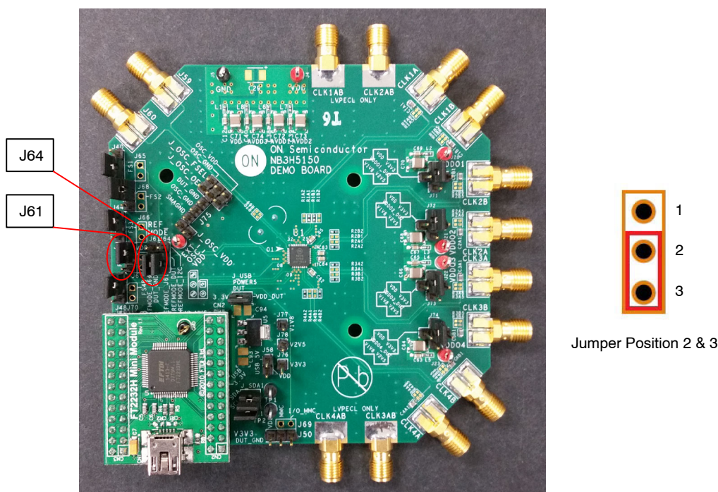
Figure 6. J61 & J64 Board Location
