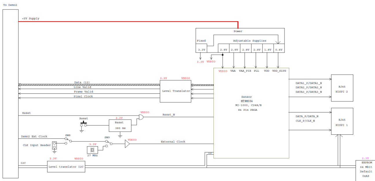
Figure 2. Block Diagram of MT9M034I12STCVH-GEVB
