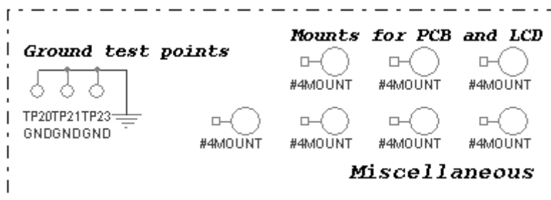
Figure 20. NCV7750 Evaluation Board Schematic – Miscellaneous Circuitry
