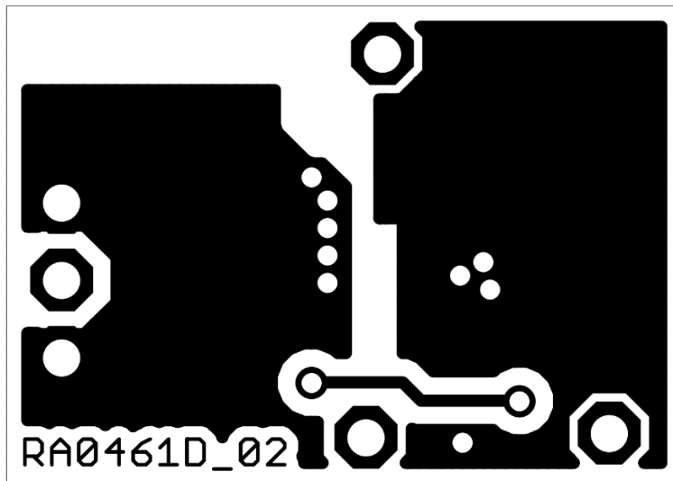
Figure 6. Bottom Layer
