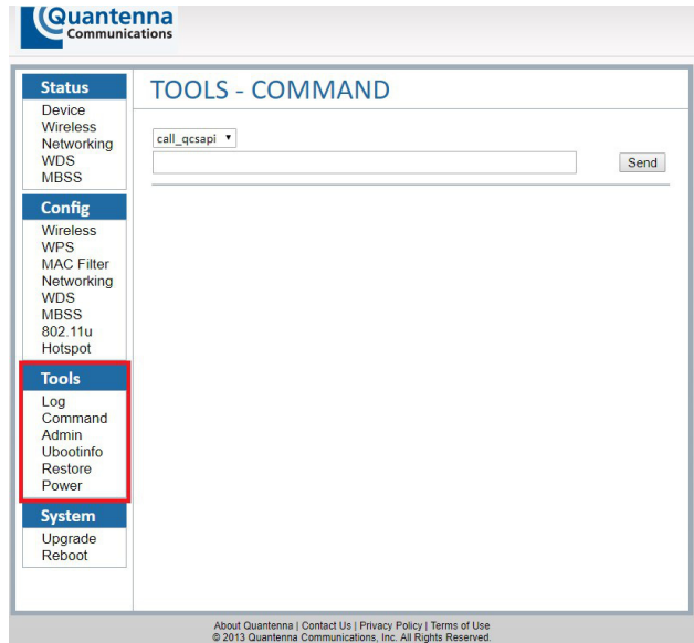
Figure 10. Tools – Command
