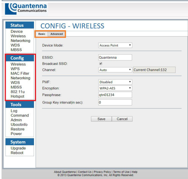
Figure 9. Config – Wireless
