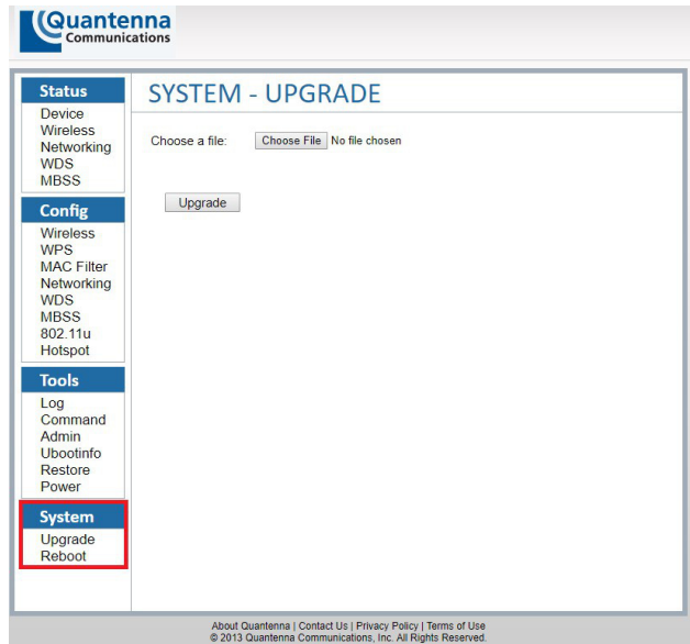
Figure 11. System – Upgrade
