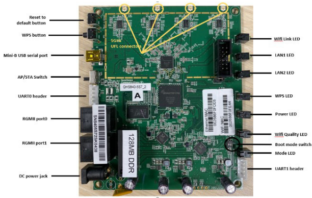
Figure 2. QHS840-5S7-GEVK Photo and Description
