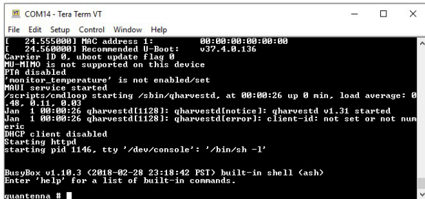
Figure 6. QHS840-5S7-GEVK Successfully Boots Up
