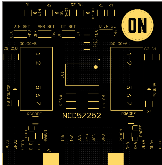
Figure 16. TOP Overlay
