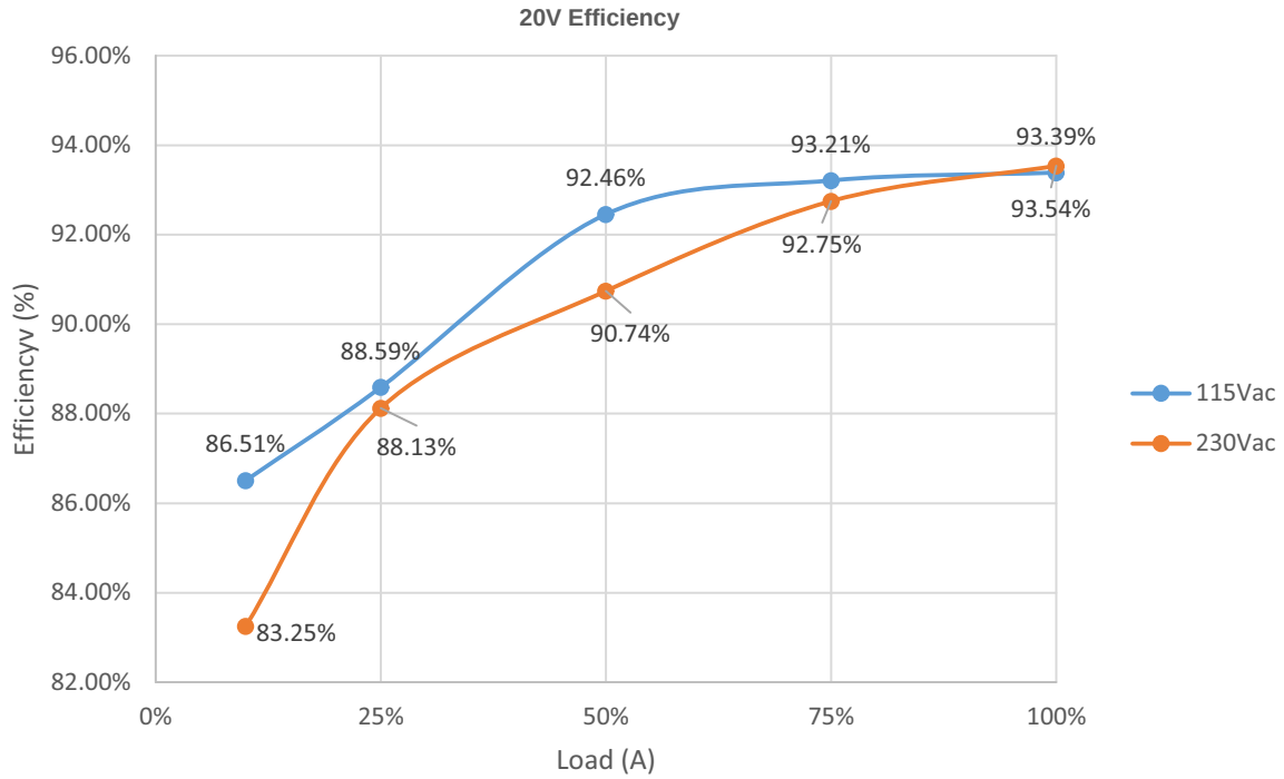
Figure 12. 20 V Efficiency
