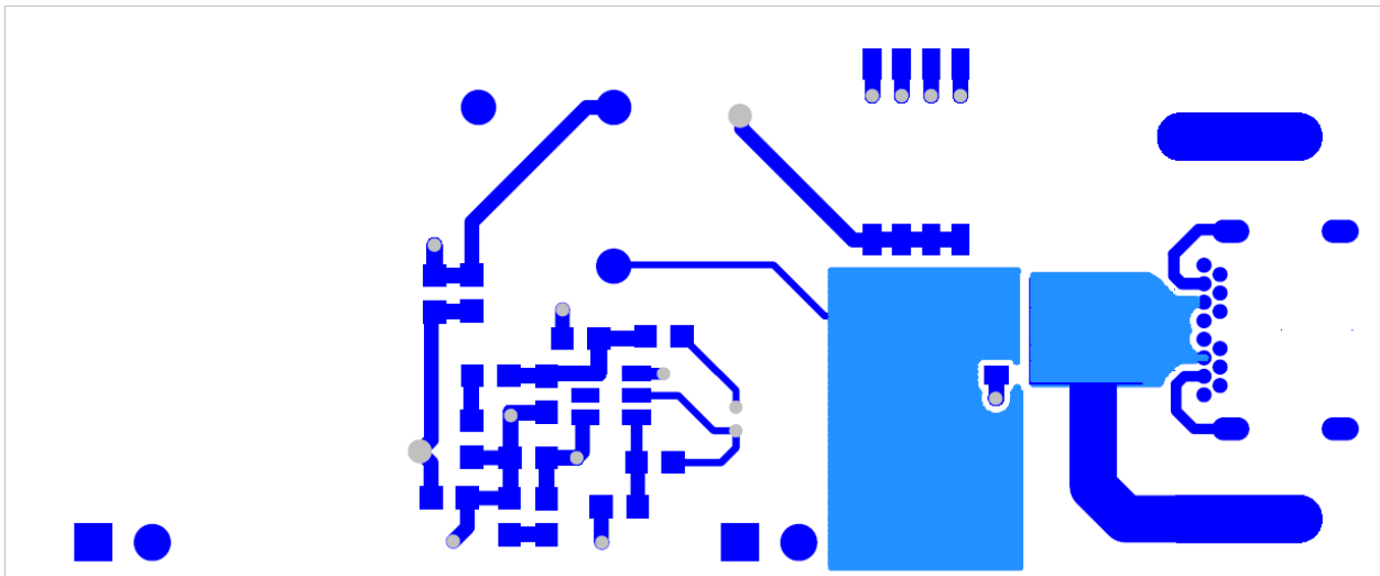
Figure 7. Top Layer
