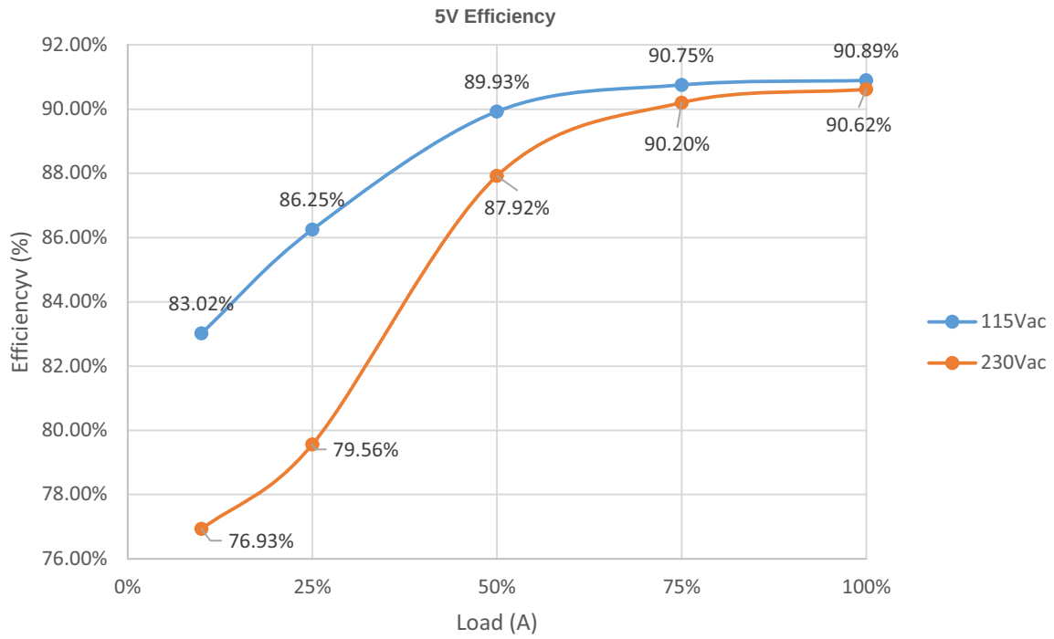
Figure 16. 5 V Efficiency
