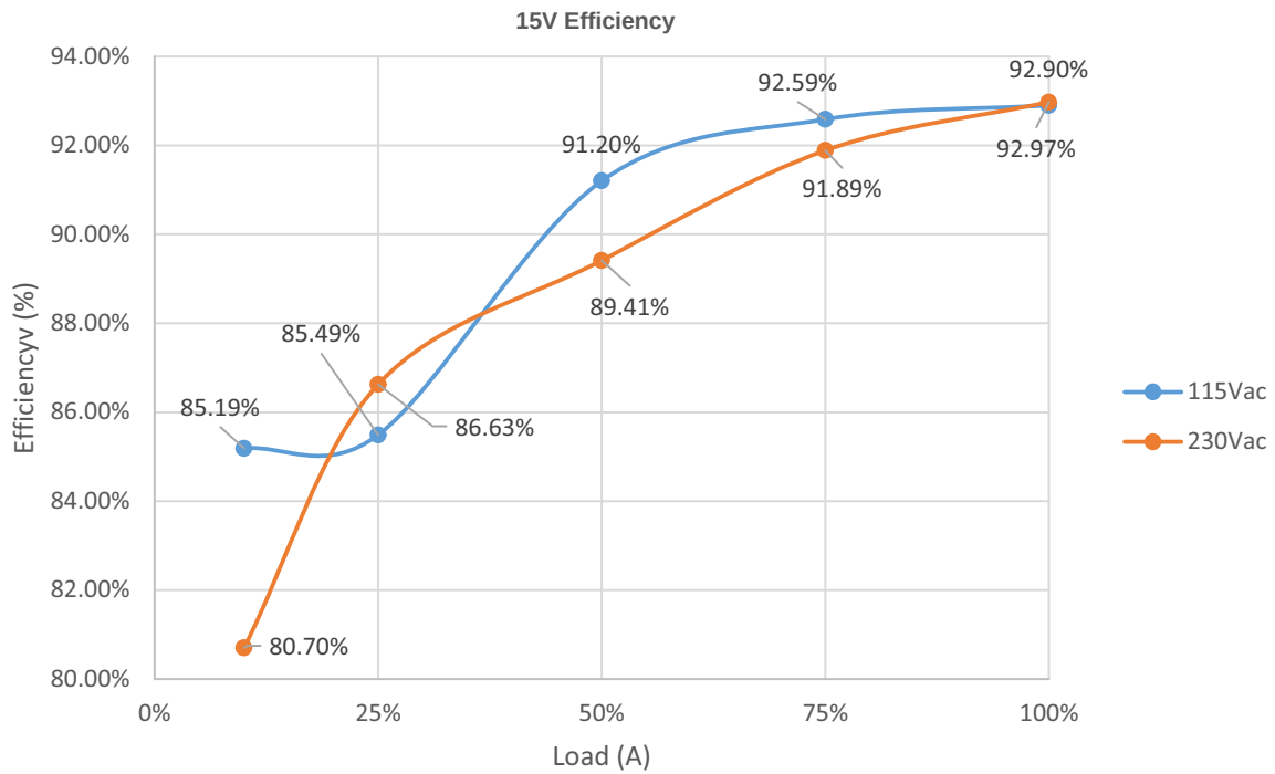
Figure 13. 15 V Efficiency
