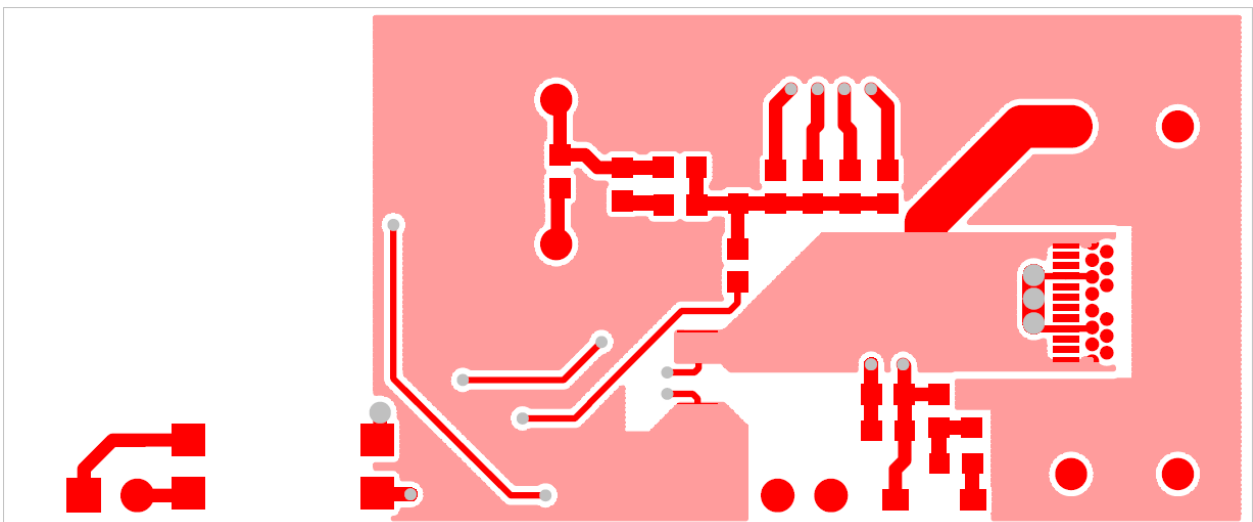
Figure 8. Bottom Layer
