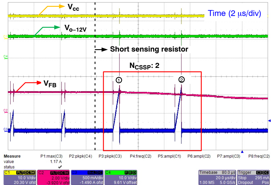
Figure 40. CSSP @ 230 V_{ac} /60 Hz, Full Load (Zoom In)
