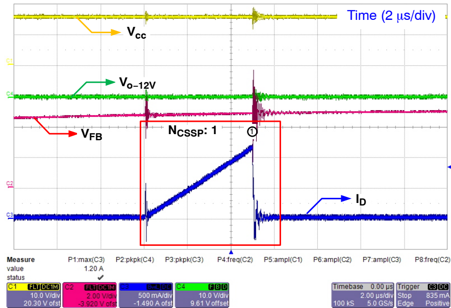
Figure 36. CSSP @ 230 V_{ac} /60 Hz, Full Load (Zoom In)
