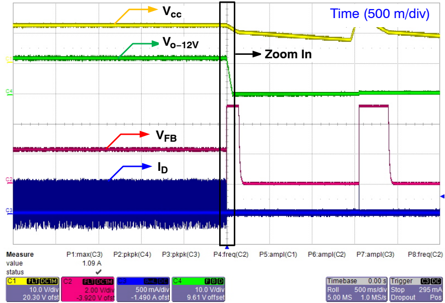
Figure 39. CSSP @ 230 V_{ac} /60 Hz, Full Load (Roll Mode)
