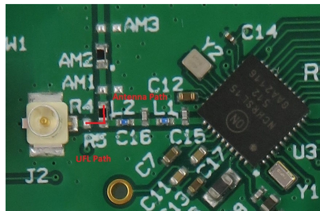
Figure 4. Selection of RF Path Through R4, R5 (0 \Omega Resistors)
