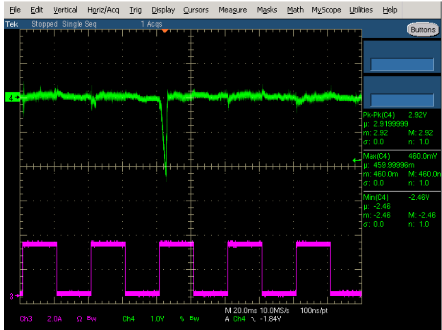
Figure 43. 57 Vin 12 Vout Transient Response
