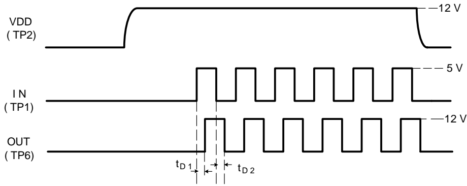
Figure 5. Timing Charts
