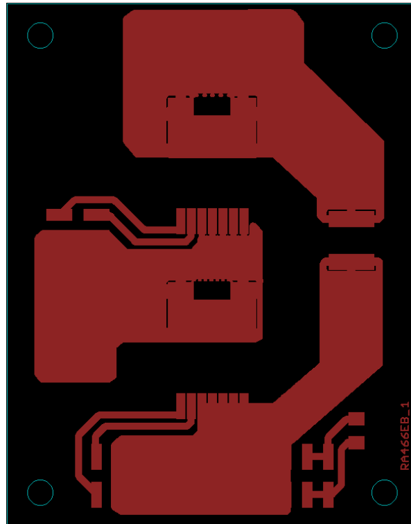
Figure 31. Top Layer
