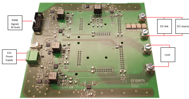
Figure 10. Board Connection
