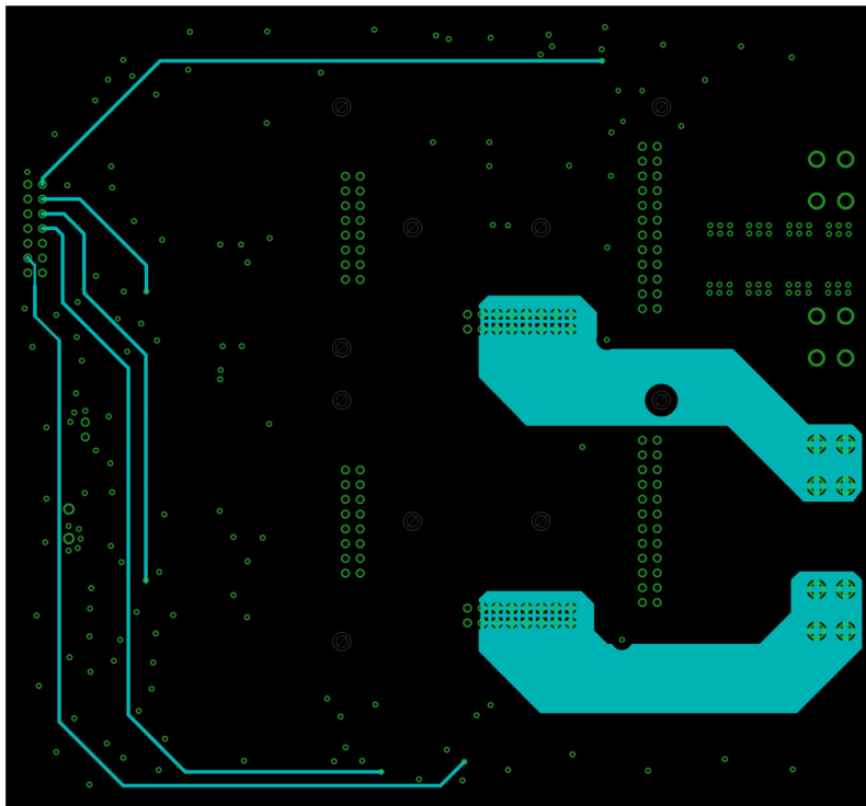
Figure 28. Signal Layer 1
