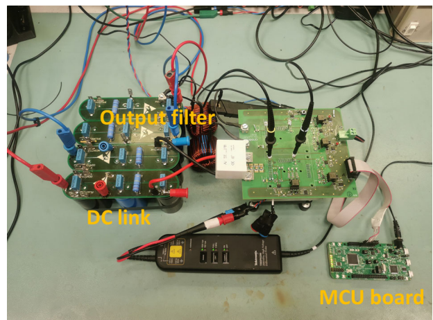
Figure 20. Application Test Setup
