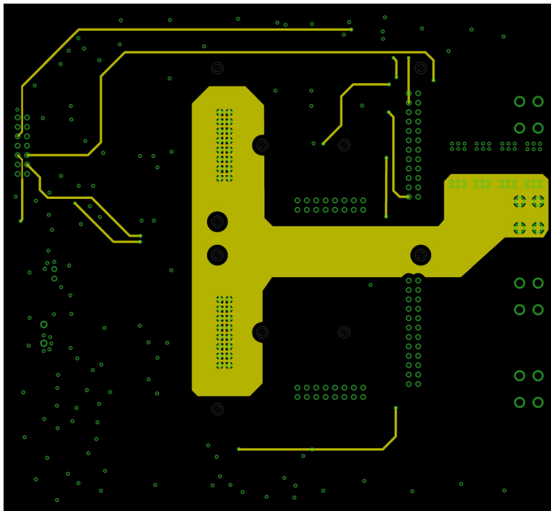
Figure 29. Signal Layer 2
