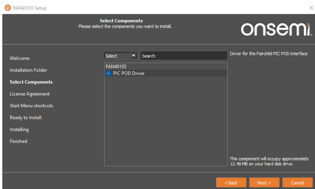
Figure 3. FAN49103 GUI Component Selection
