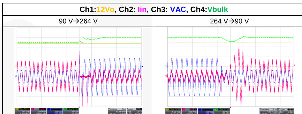
Figure 18. Test Waveform of AC Trim Up & Trim Down
