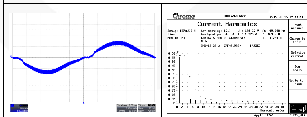
Figure 13. Input Current Waveform and THD Test Result in 115 V AC , Mid. Load
