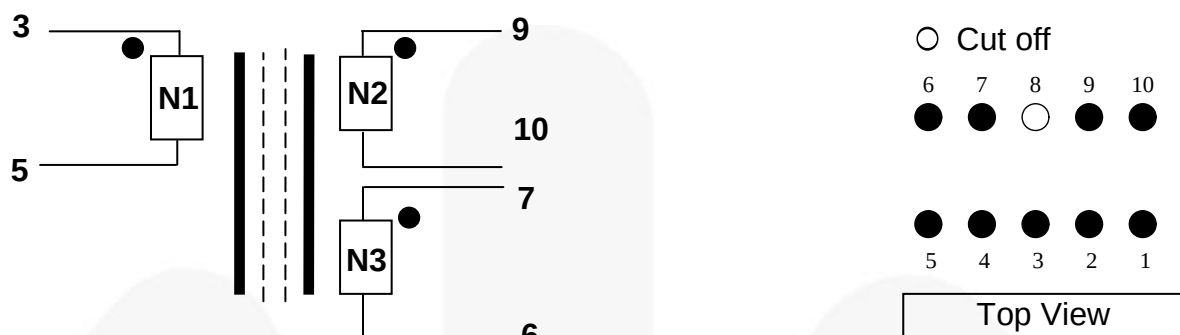
Figure 7. Transformer Specifications of TX2
