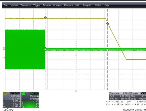
Figure 34. t_{HOLD} = 8.8 \text{ s} , 460 V AC , (CH1: V_{OUT} (5 V/div), CH4: V AC (350 V/div), Time: 2 s/div)
