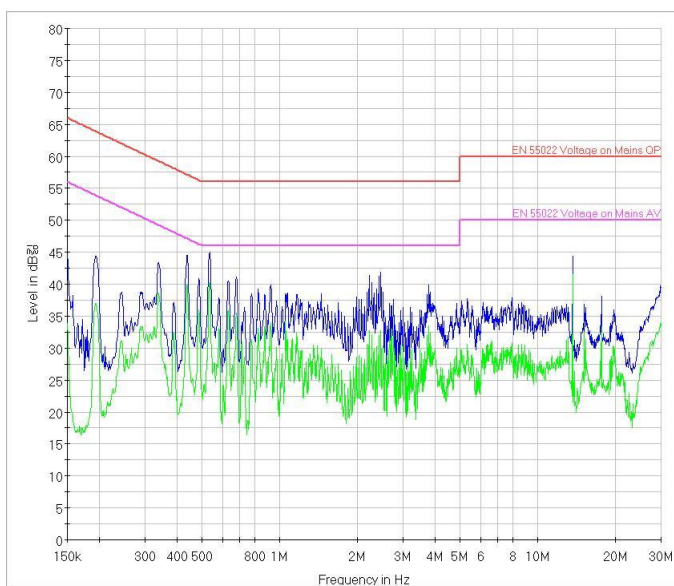
Figure 43. Conduction Neutral: 110 V AC
