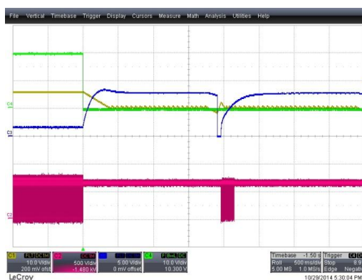
Figure 36. OLP Triggered, Output Short with 460 V AC , Full-Load, (CH1: V CC (10 V/div), CH2: V DS (500 V/div), CH3: V FB (5 V/div), CH4: V OUT (10 V/div), Time: 500 ms/div)
