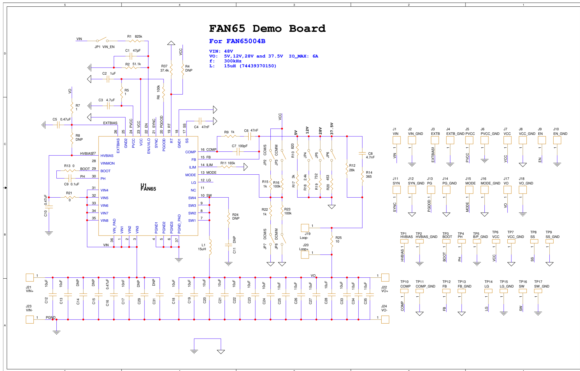
Schematic for the FAN65004B-GEVB Evaluation Board
