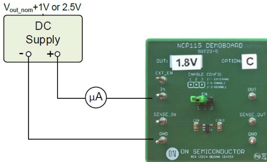
Figure 1: Test configuration for measurement I_Q , Quiescent Current
