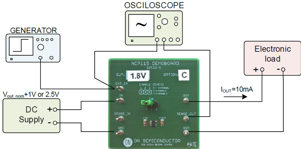
Figure 4: Test configuration for measurement enables response
