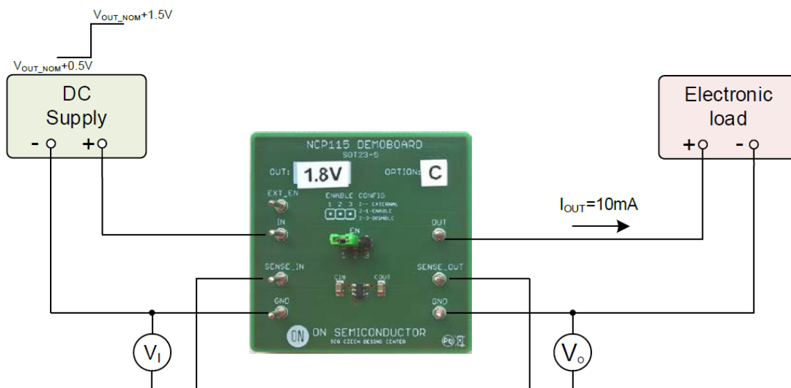
Figure 3: Test configuration for measurement REG_{LINE} , Line Regulation
