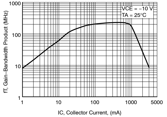
Figure 9. fT – IC
