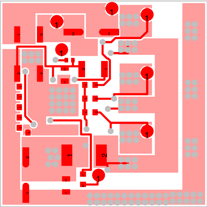
Figure 7. Bottom Layer
