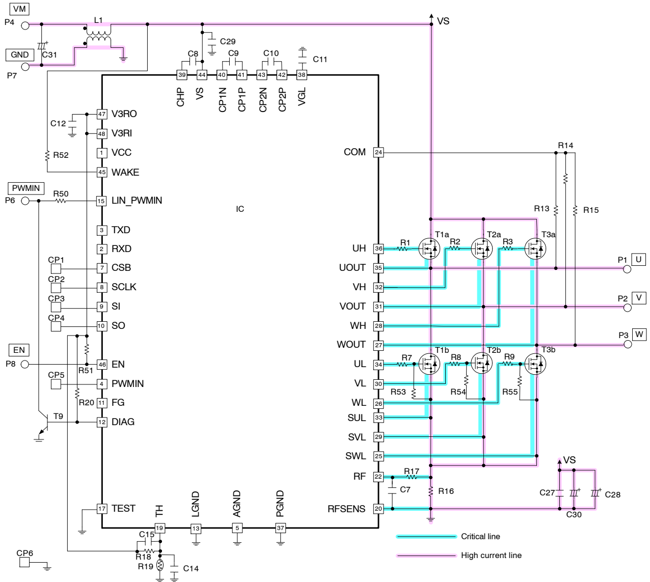
Figure 2. Schematic
