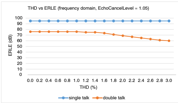
Figure 12. THD vs ERLE (Frequency Domain, Echo Cancel Level = 1.05)
