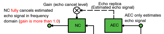
Figure 3. Frequency Domain Mode
