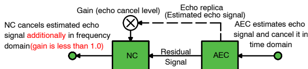
Figure 2. Time Domain Mode
