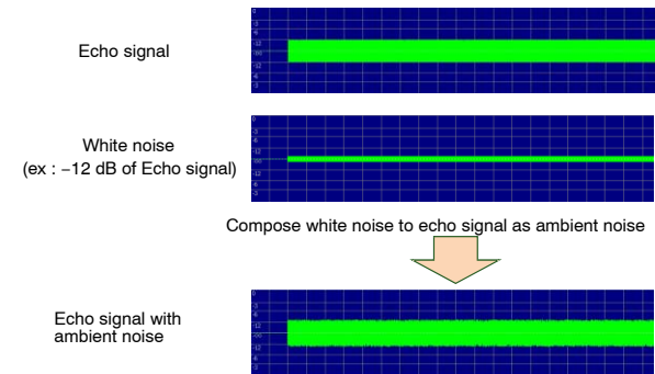
Figure 5. Echo Signal with Ambient Noise
