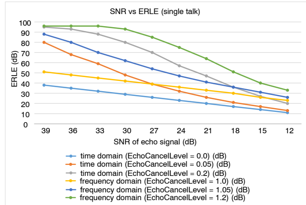
Figure 21. Ambient Noise vs ERLE (Single Talk)
