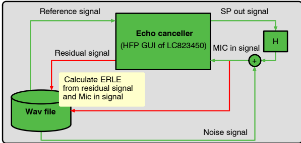
Figure 4. Overview of PC Simulation
