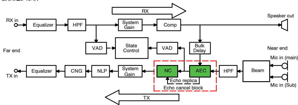
Figure 1. Block Diagram of HFP Program of LC823450
