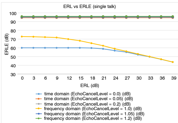
Figure 14. ERL vs ERLE (Single Talk)
