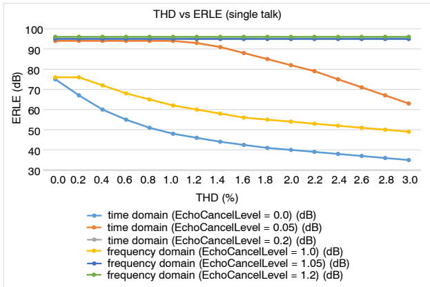
Figure 7. THD vs ERLE (Single Talk)
