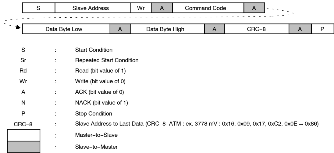
Figure 22. Write Word Protocol
