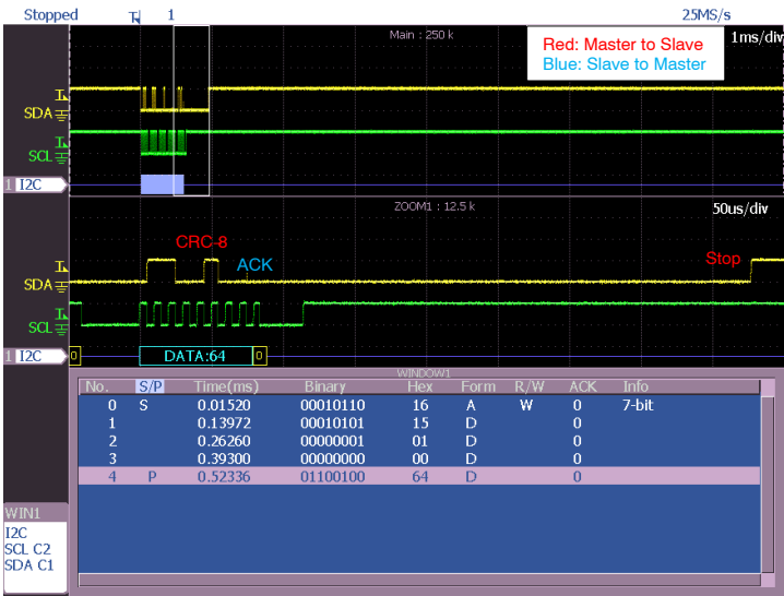
Figure 26. Write Waveform (3)
