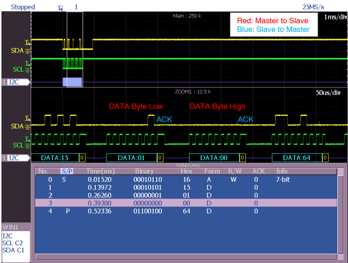
Figure 25. Write Waveform (2)
