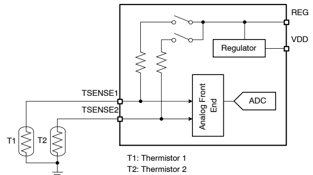
Figure 4. TSENSE1/TSENSE2 Port Block Diagram
