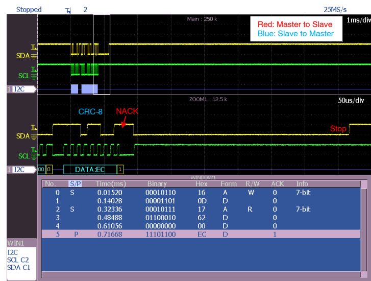
Figure 21. Read Waveform (3)
