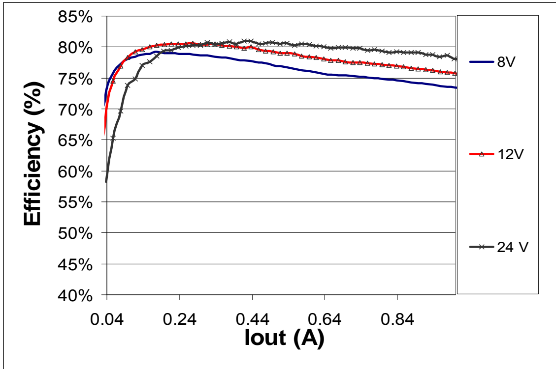
Figure 5– NCP3063 Efficiency 8V-24V with at 5V output Voltage.
