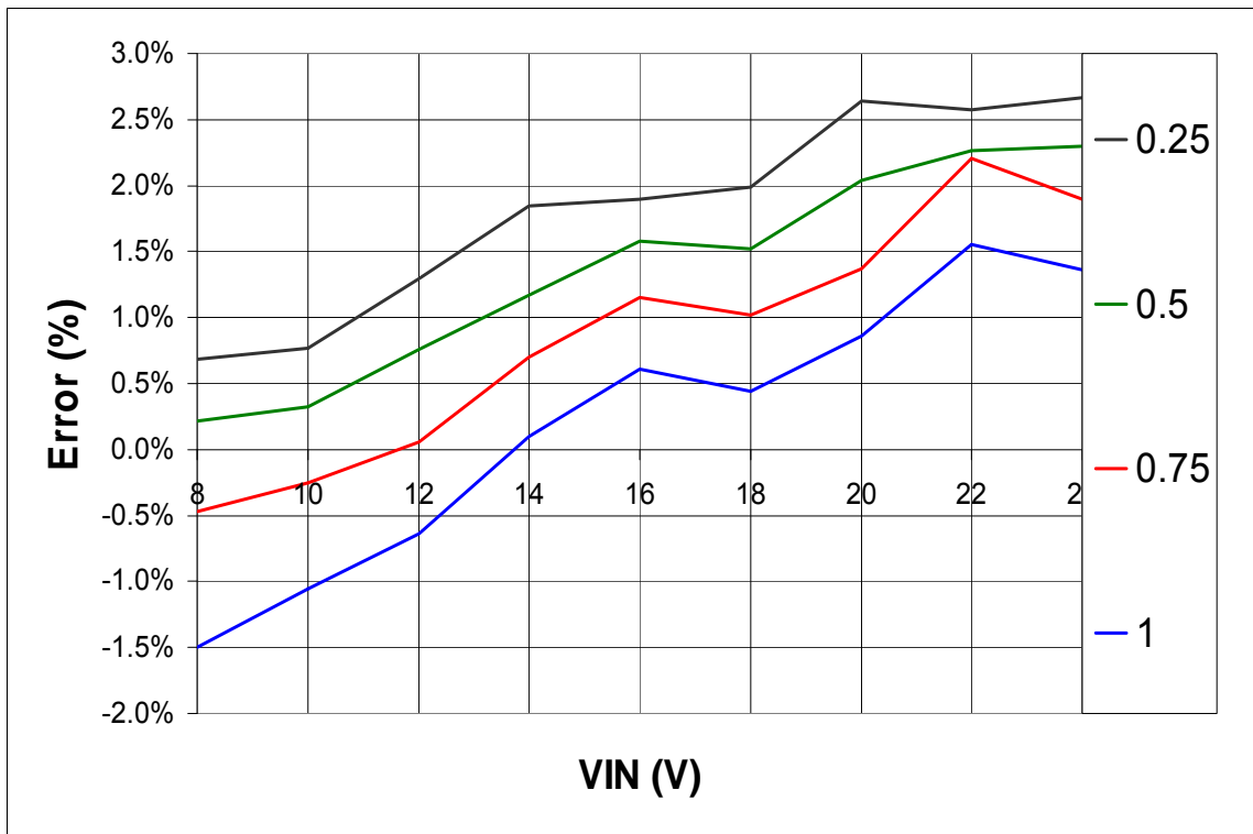
Figure 9 - NCP3063 Line Regulation Error
