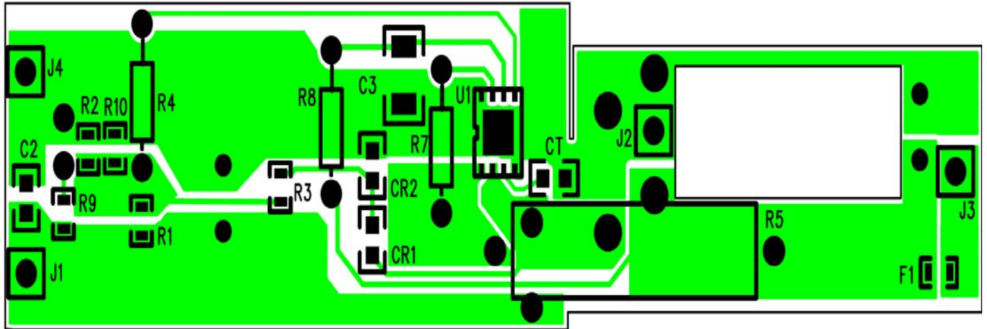
Figure 1 – NCP3063 CLA Top Layout and Silkscreen
