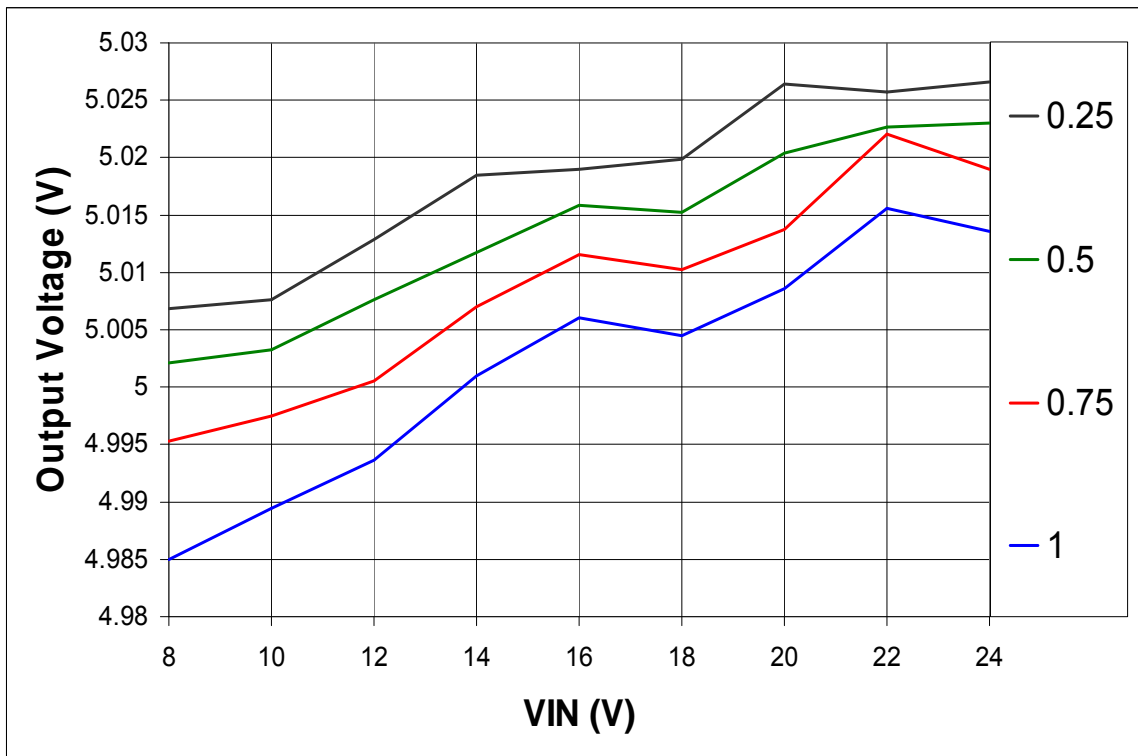
Figure 8 - NCP3063 Line Regulation
