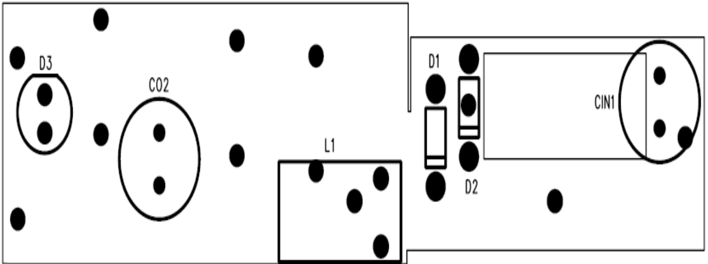
Figure 2 – NCP3063 Bottom Layout and Silkscreen
