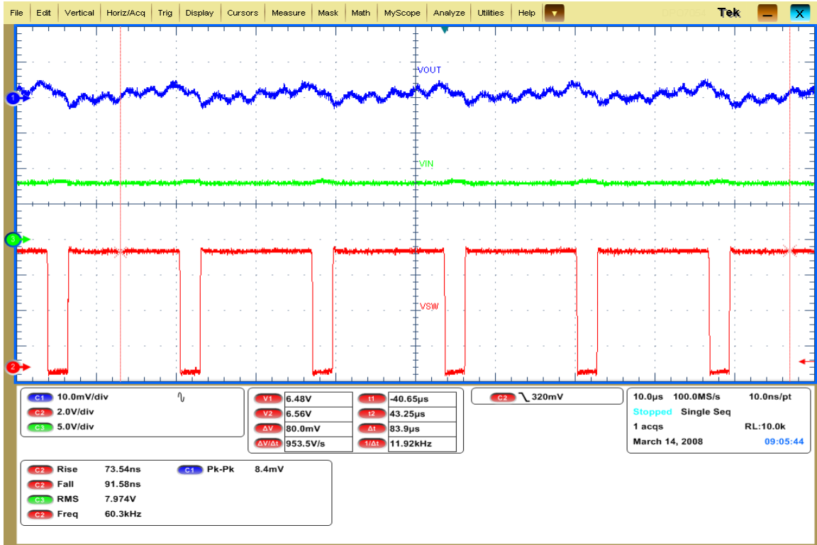
Figure 12- NCP3063 Output Ripple at 8 V to 5 V at a 1 A Load
