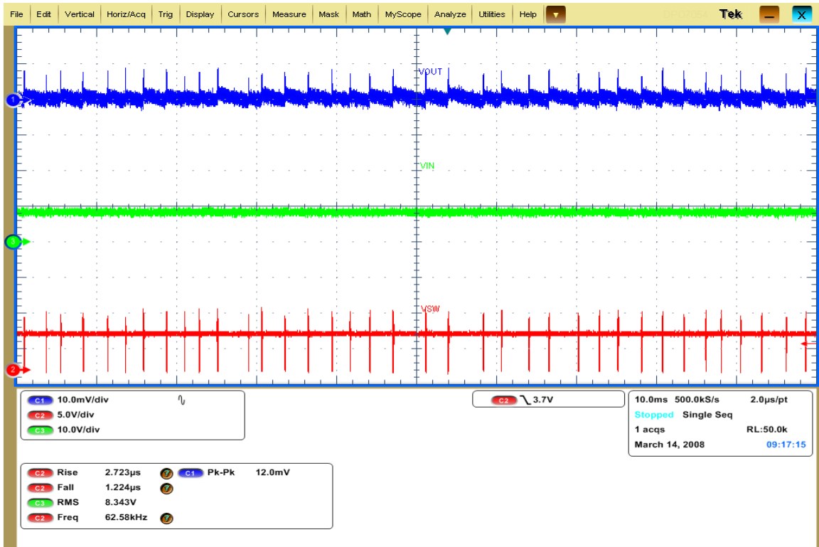
Figure 13- NCP3063 Output Ripple at 8 V to 5 V at a no load
