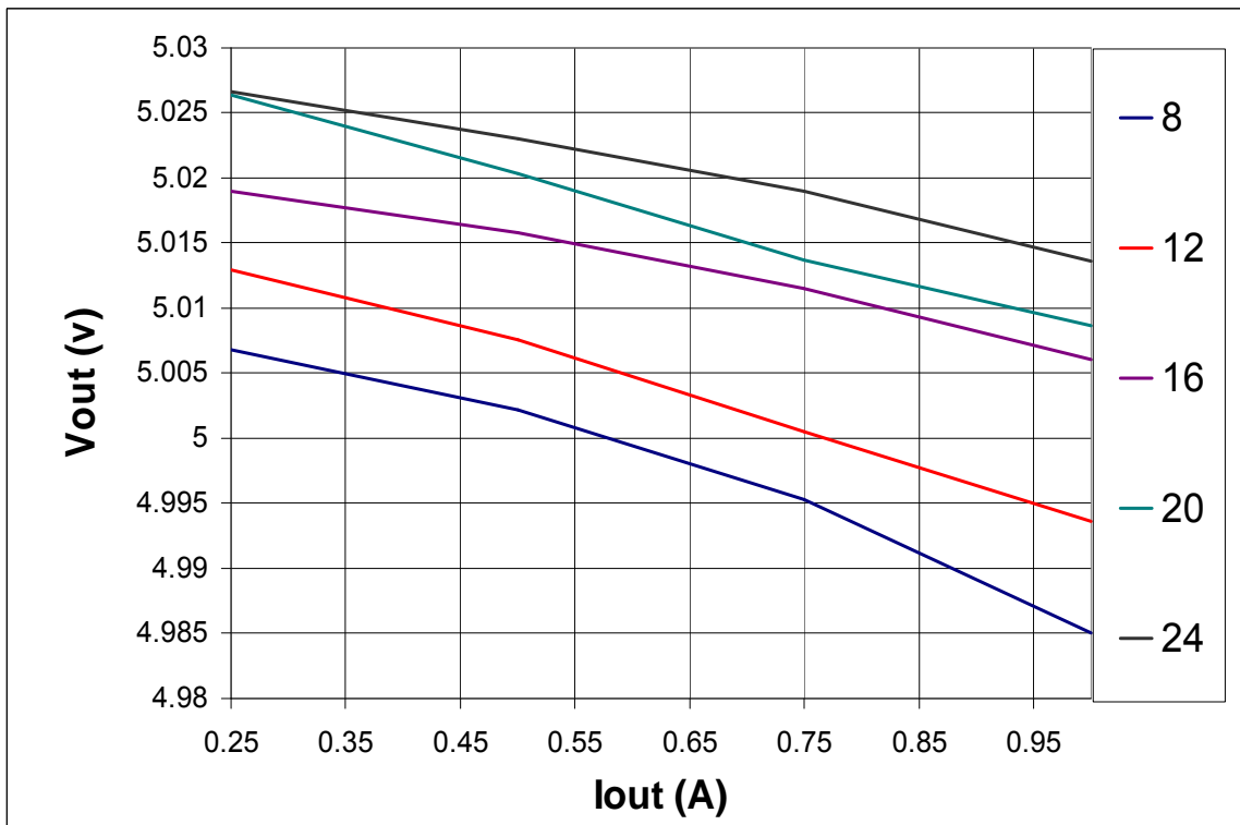
Figure 6 – NCP3063 Load Regulation
