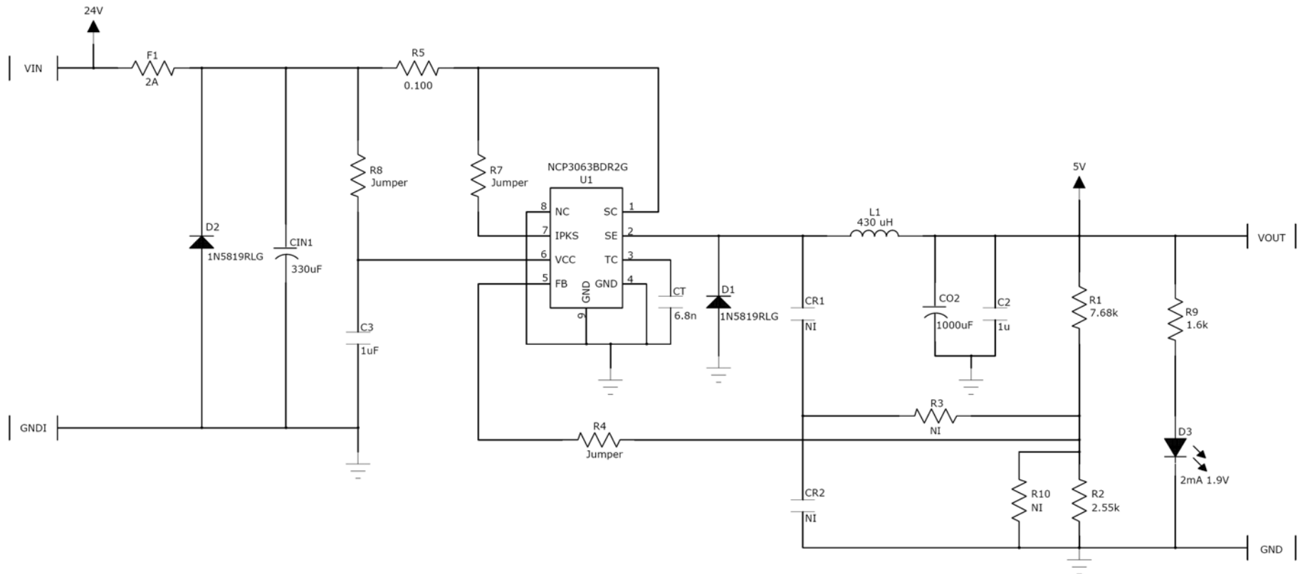
Figure 3 – NCP3063 Schematic
