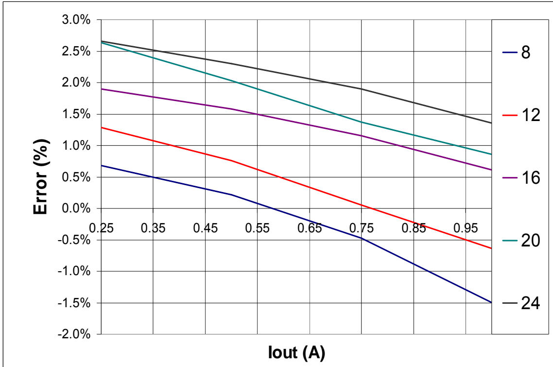
Figure 7 - NCP3063 Load Regulation Error
