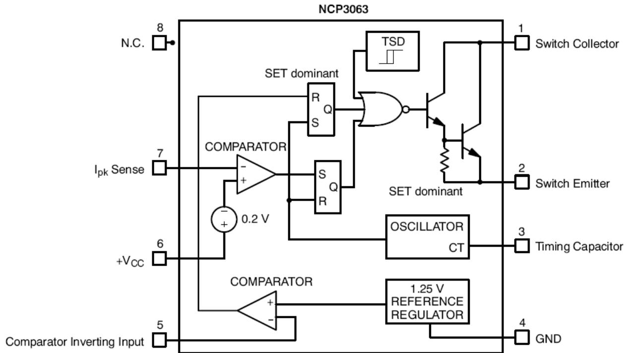
Figure 4 – NCP3063 Block Diagram
