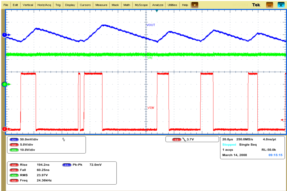
Figure 10- NCP3063 Output Ripple at 24 V to 5 V at a 1 A Load
