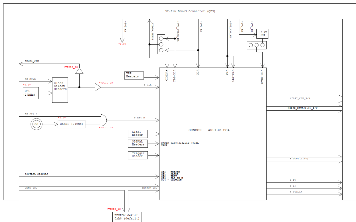
Figure 2. Block Diagram of AR0132AT6M00XPEAH3-GEVB
