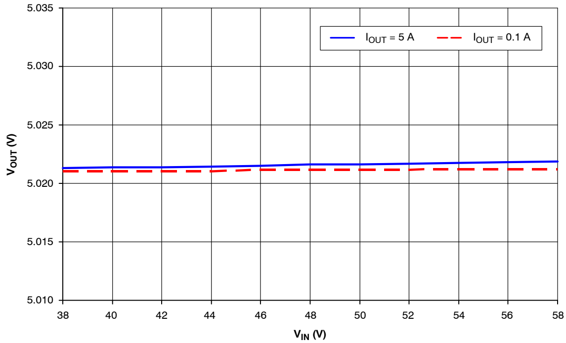
Figure 22. Line Regulation
