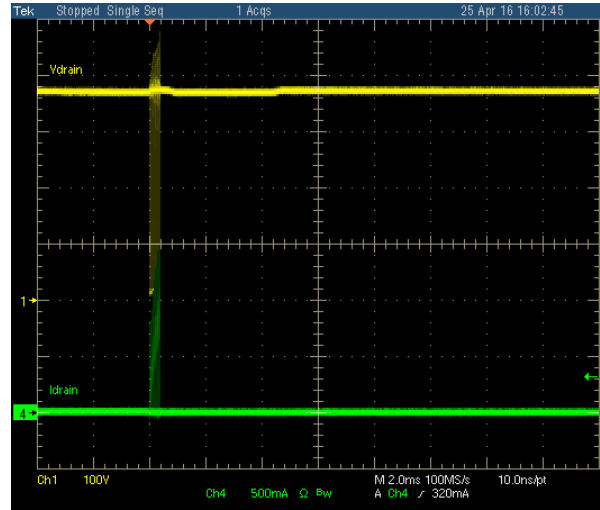
Figure 24. 265 Vac Short-circuit
