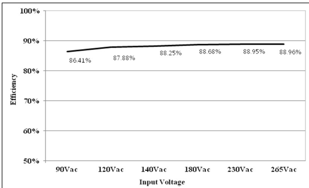
Figure 28. System Efficiency
