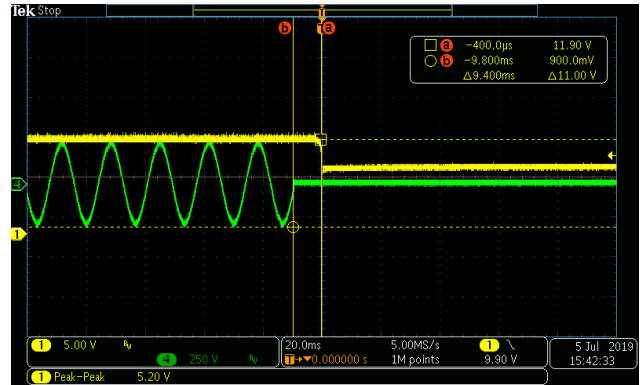
Figure 10. Hold-up Time
