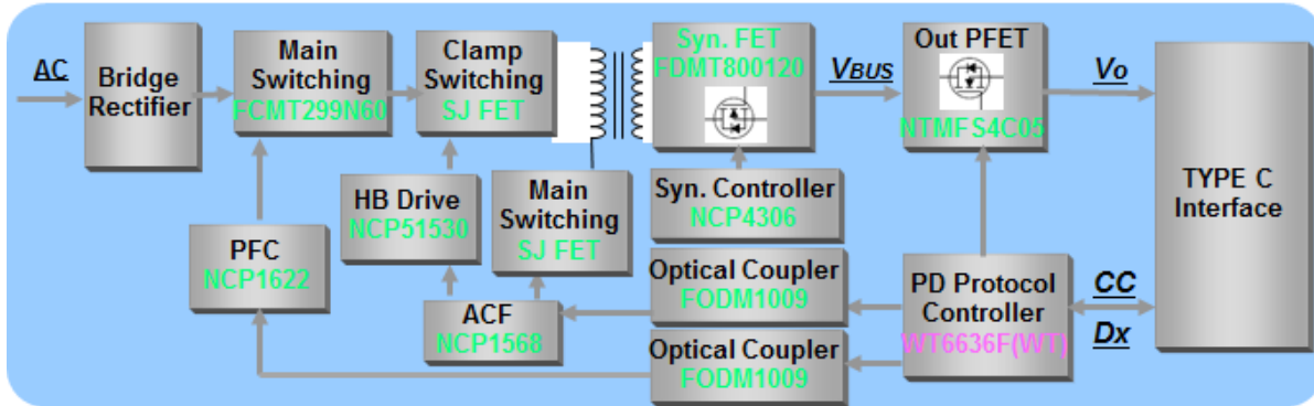
Figure 1. Overall Cycle of 90 W TYPE-C PD Adapter Solution
