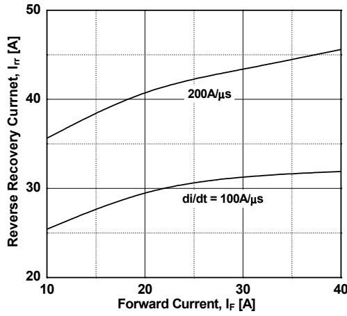
Figure 19. Reverse Current
