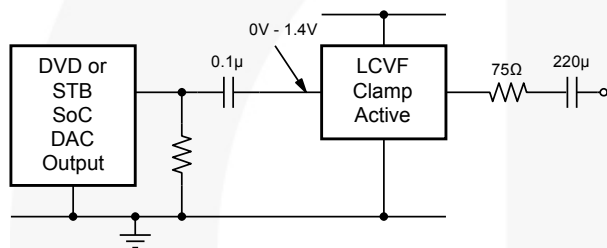
Figure 17. DC-Coupled Inputs, AC-Coupled Outputs
