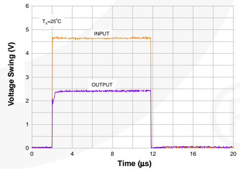
Figure 16. Pulse Response
