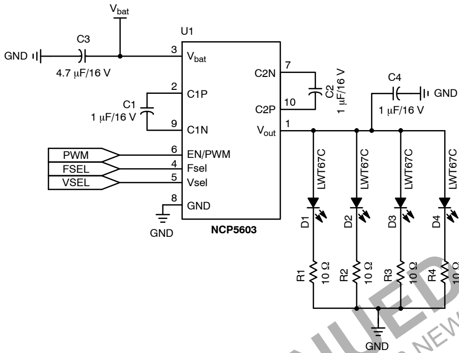
Figure 1. Typical Application
