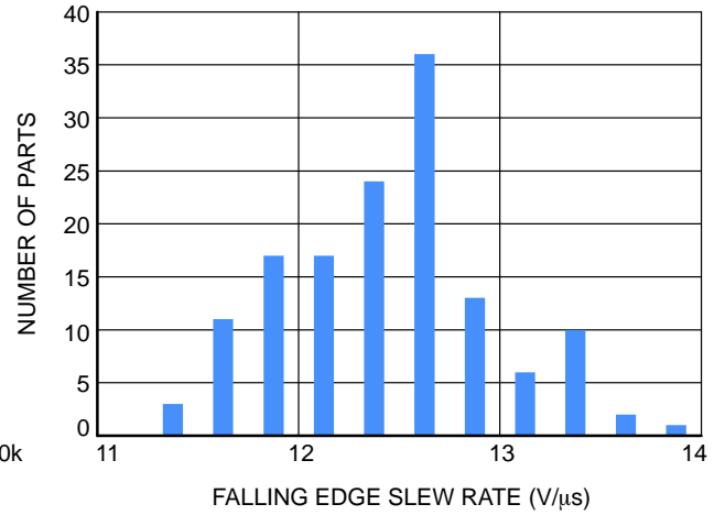
Figure 23. Falling Edge Slew Rate @ V_S = 5\text{ V}
