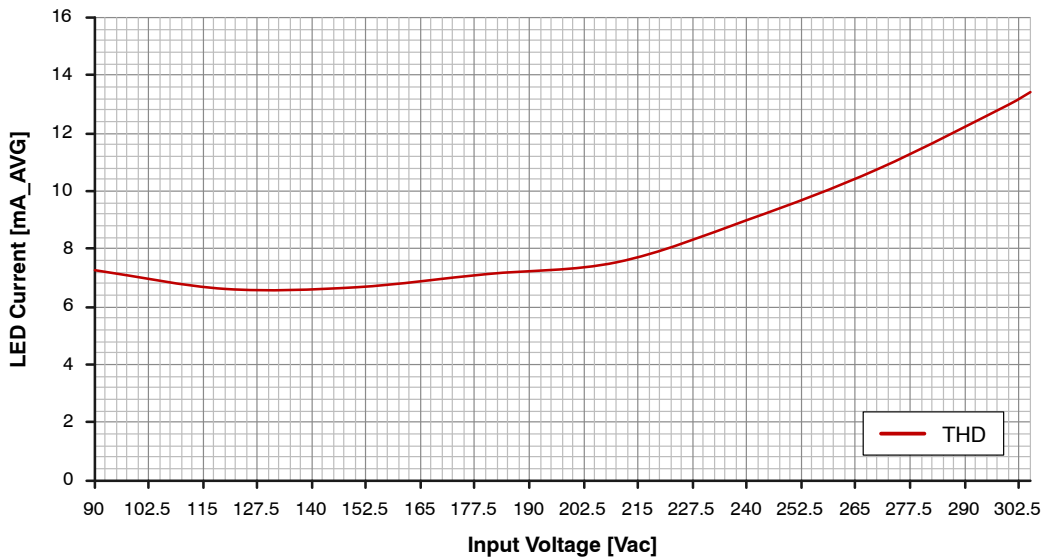
Figure 10. THD Performance
