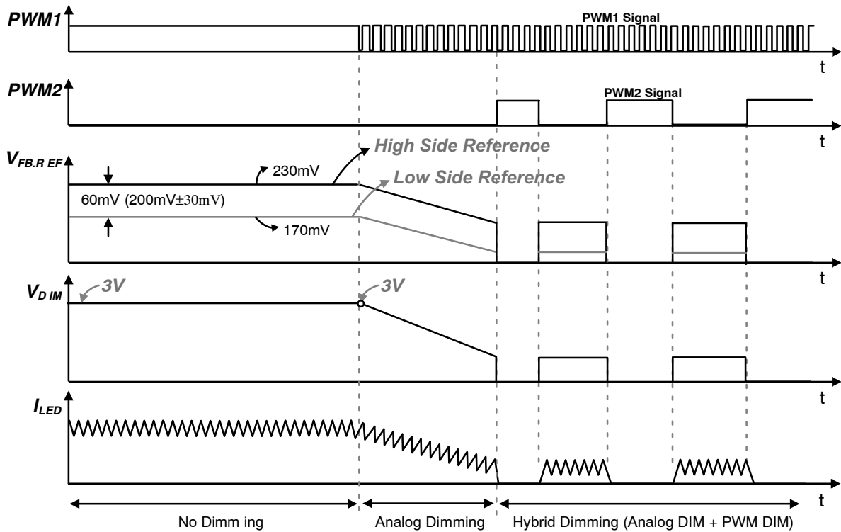
Figure 12. Hybrid Dimming Performance
