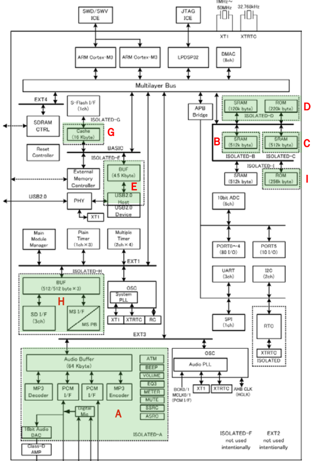
Figure 3. Isolation blocks
