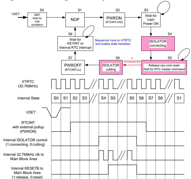
Figure 5. State diagram of Keyint RTC mode
