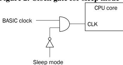
Figure 2. Clock gate for sleep mode
