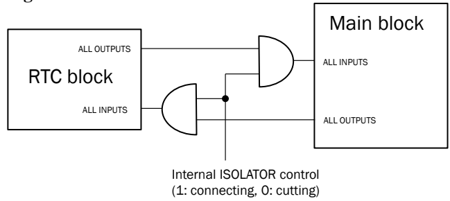
Figure 4. Isolation control
