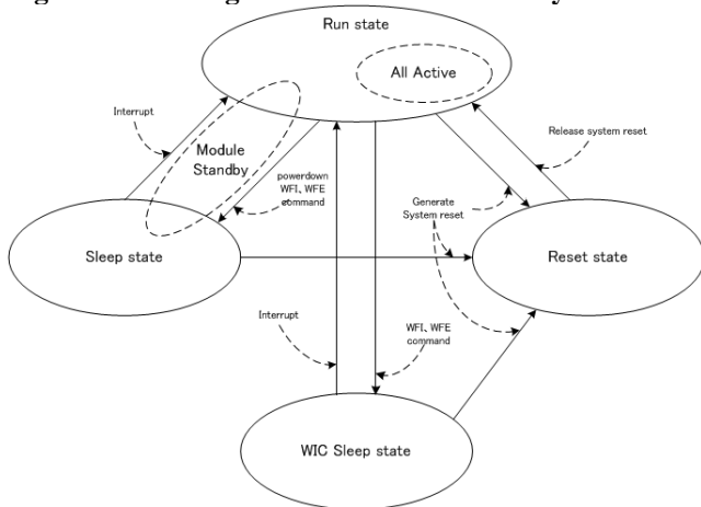
Figure 1. Working state transition of OSC system
