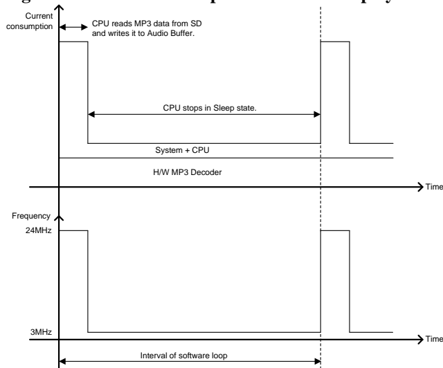
Figure 6. Current consumption at H/W MP3 playback
